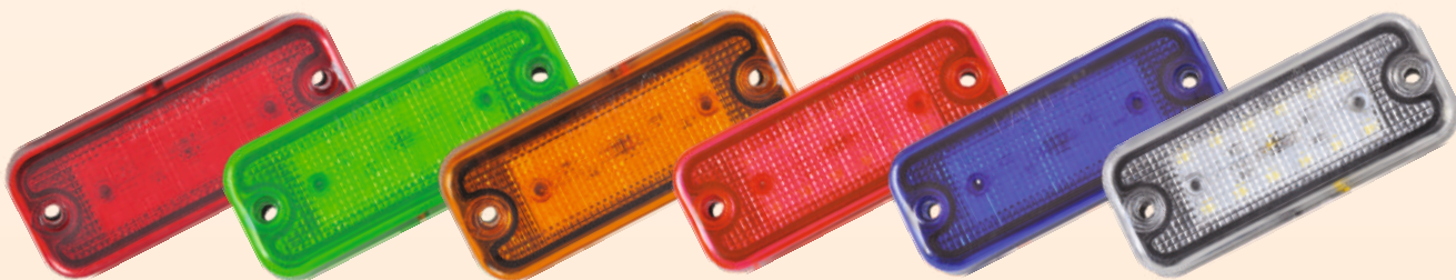
PAL-SI-SKT 3600 R|G|Y|B|W|P Waterproof 98x40mm 12v|24v
