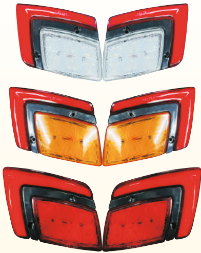
PAL-TL-219 192X105 MM 12V/24V R/Y/W
